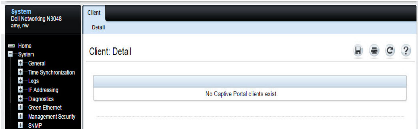
Figure 9-36. Client
