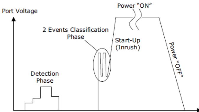
Figure 2-1. PD Detection
