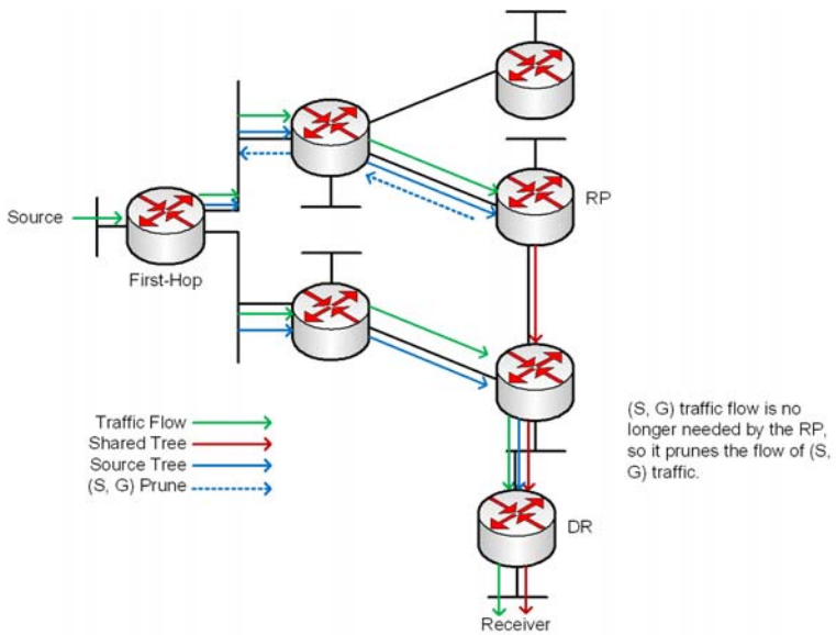
Figure 46-7. PIM-SM SPT—Part 4
