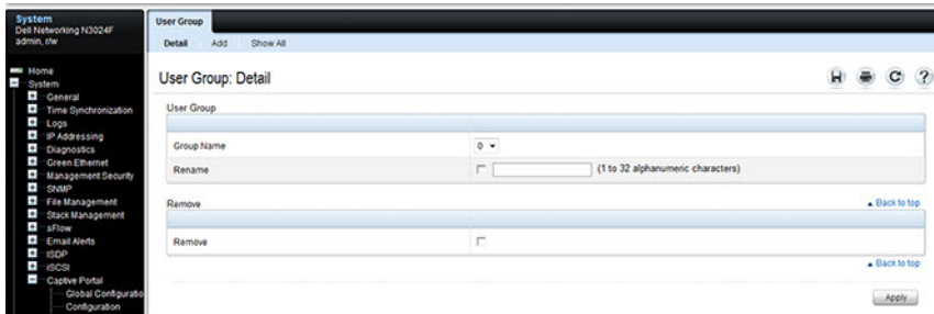
Figure 9-27. User Group
