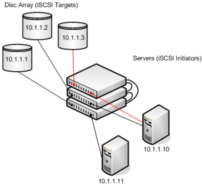
Figure 16-2. iSCSI Optimization
