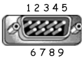
Male DSUB 9-Pin
