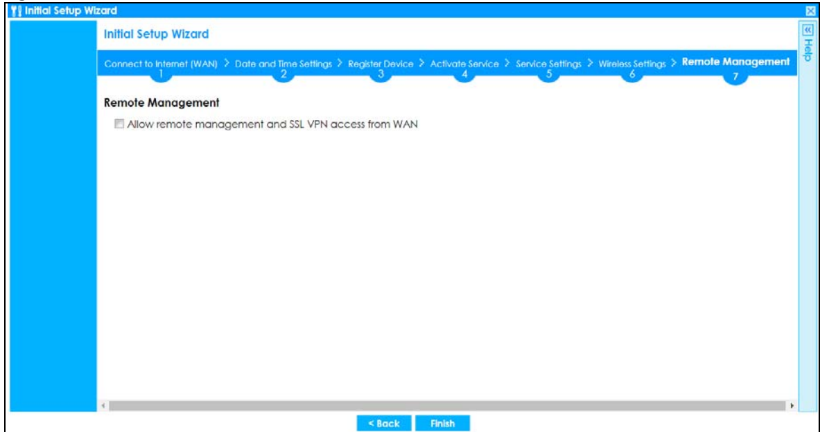
Figure 39 Remote Management
