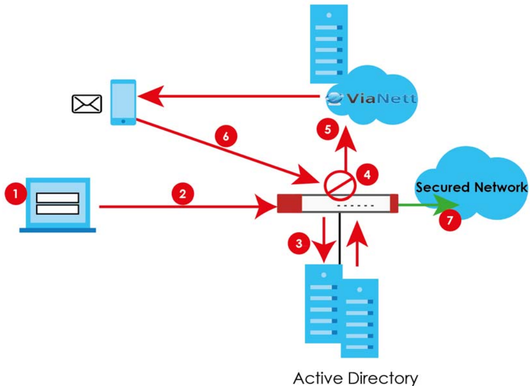
Figure 426 Two-Factor Authentication
