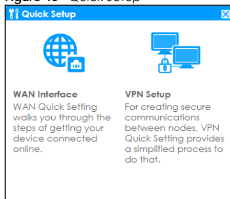
Figure 46 Quick Setup
