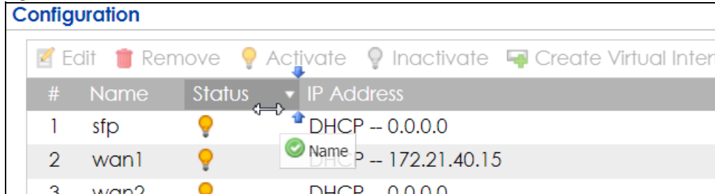
Figure 18 Moving Columns
