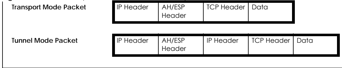
Figure 280 VPN: Transport and Tunnel Mode Encapsulation
