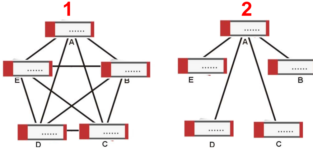
Figure 272 VPN Topologies (Fully Meshed and Hub and Spoke)
