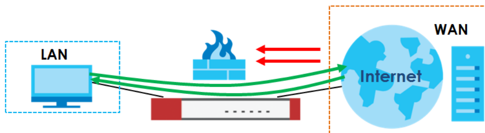
Figure 321 Default Directional Security Policy Example
