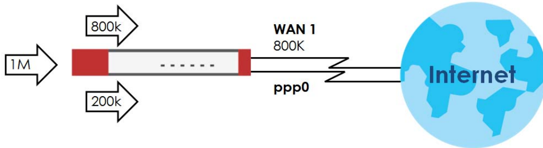
Figure 197 Spillover Algorithm Example
