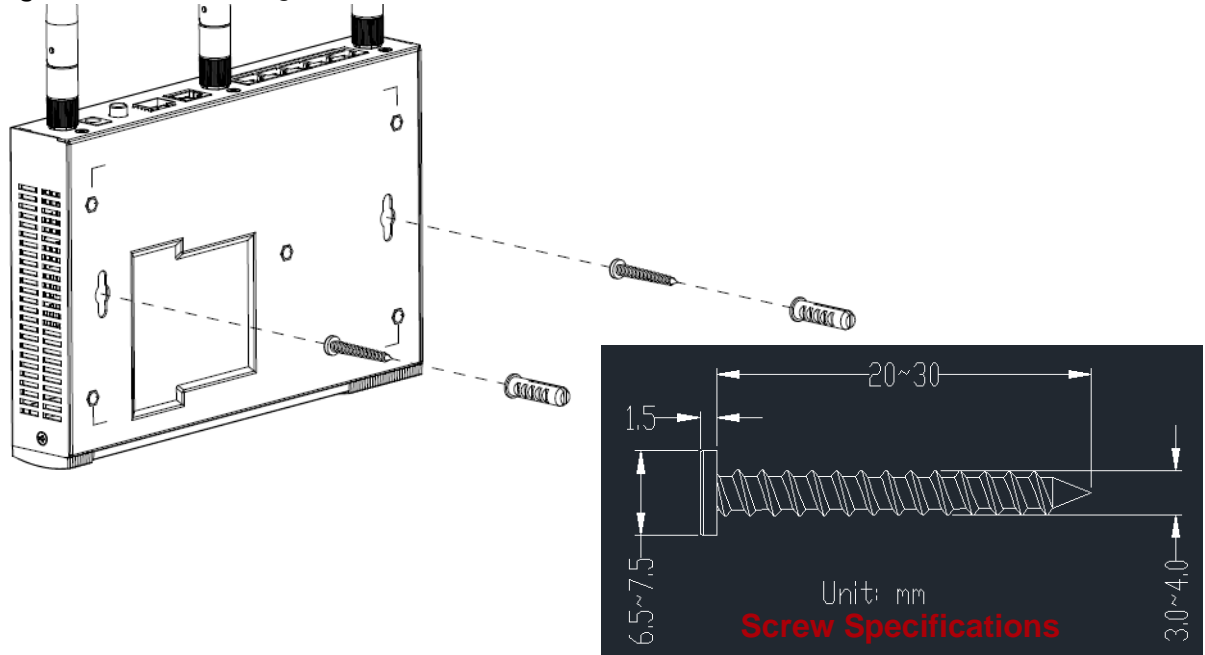
Figure 45 Wall Mounting
