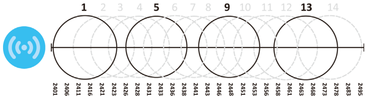
Figure 162 An Alternative Four-Channel Deployment
