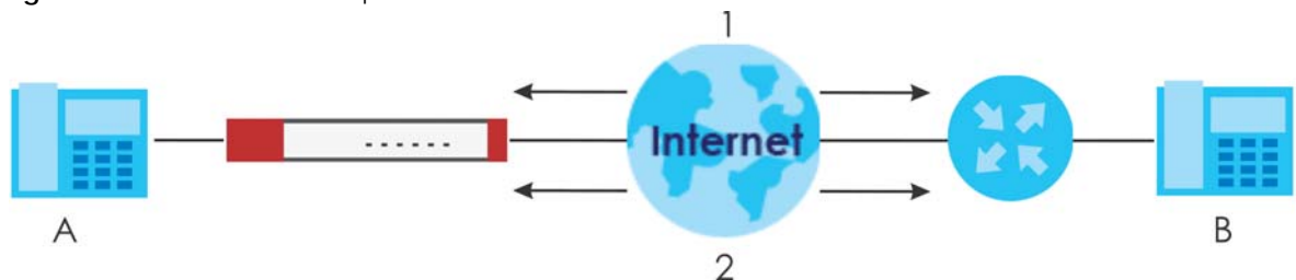
Figure 235 H.323 ALG Example
