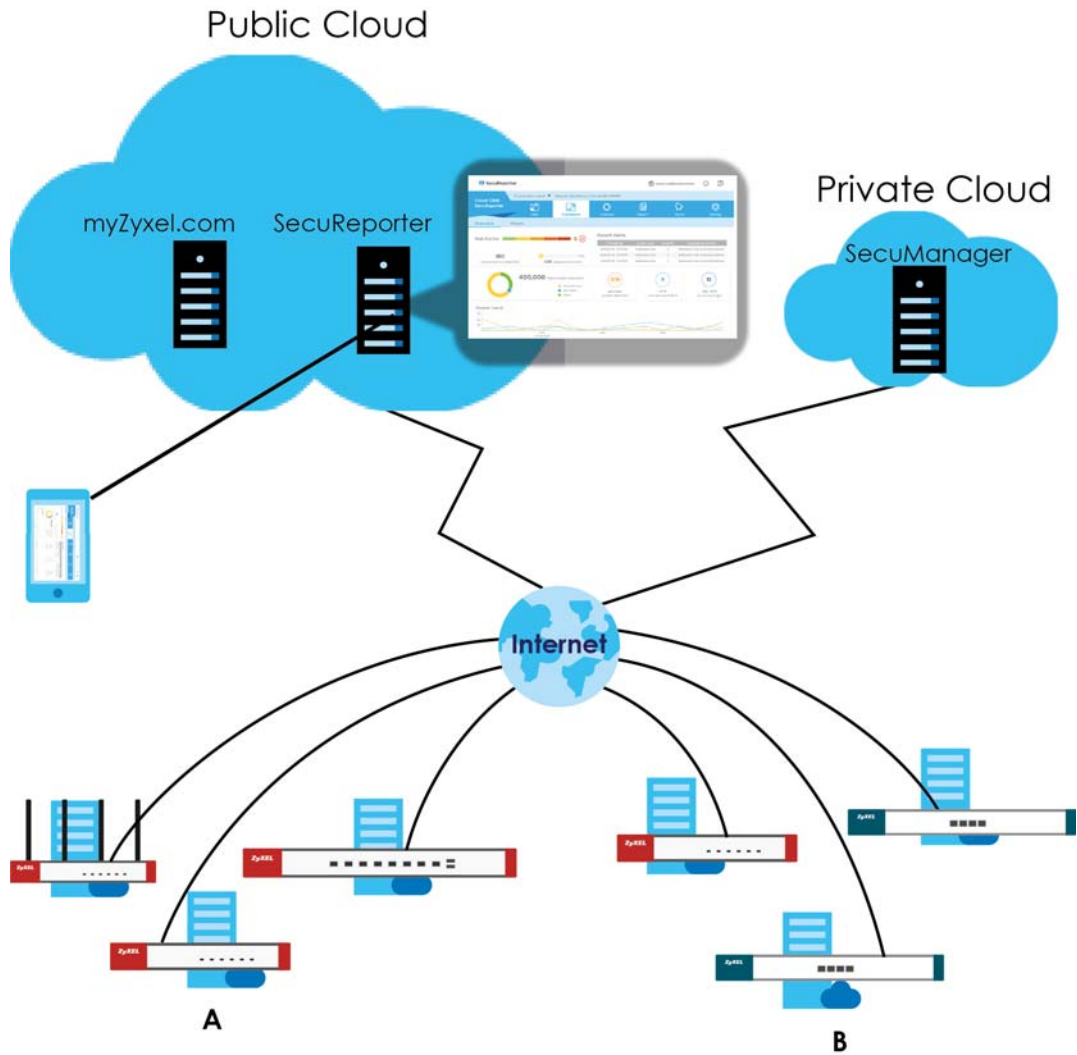
Figure 450 Cloud CNM SecuReporter Application Scenario
