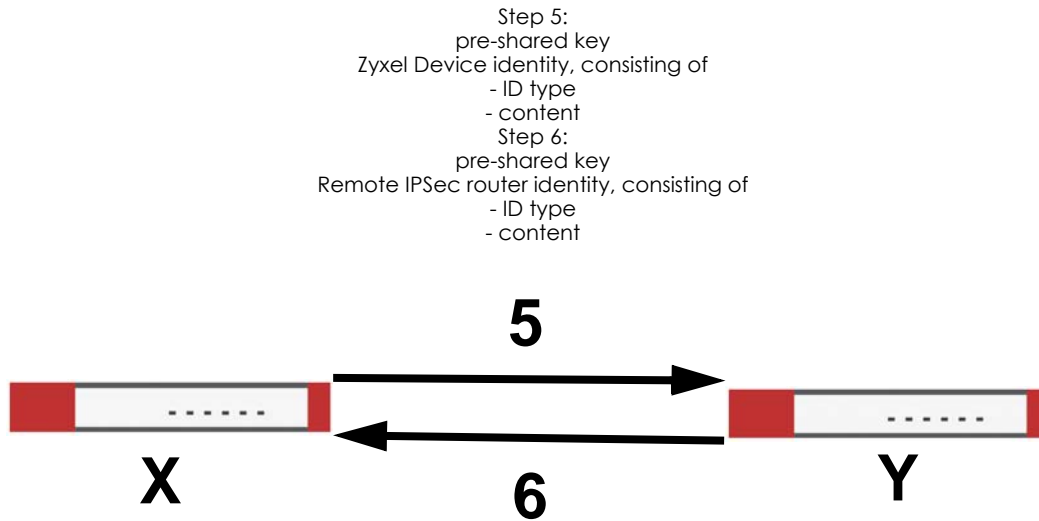
Figure 278 IKE SA: Main Negotiation Mode, Steps 5 - 6: Authentication (continued)
