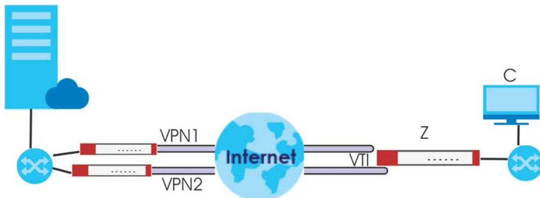
Figure 192 VTI and Trunk for VPN Load Balancing
