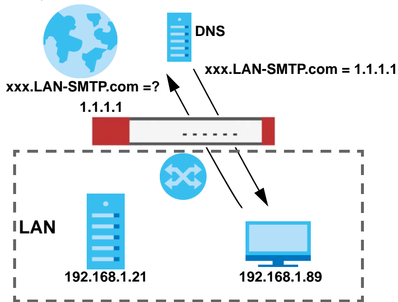
Figure 227 LAN Computer Queries a Public DNS Server
