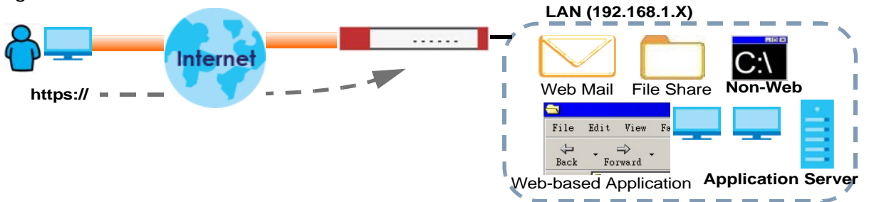
Figure 5 SSL VPN With Full Tunnel Mode
