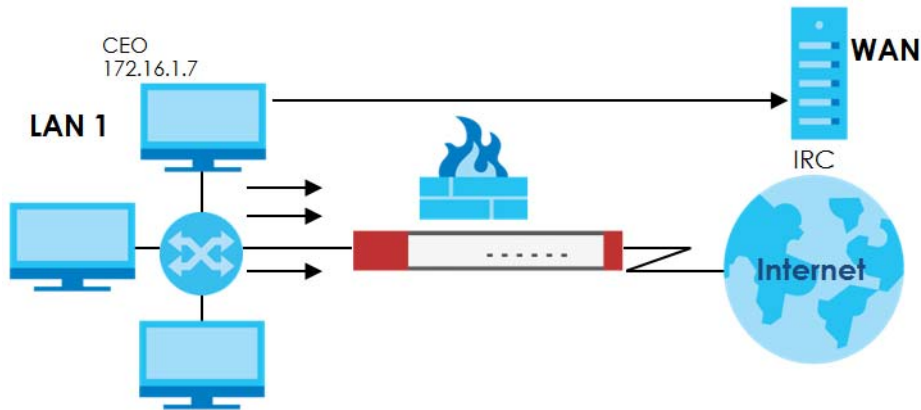
Figure 335 Limited LAN to WAN IRC Traffic Example
