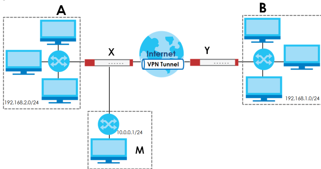
Figure 281 VPN Example: NAT for Inbound and Outbound Traffic
