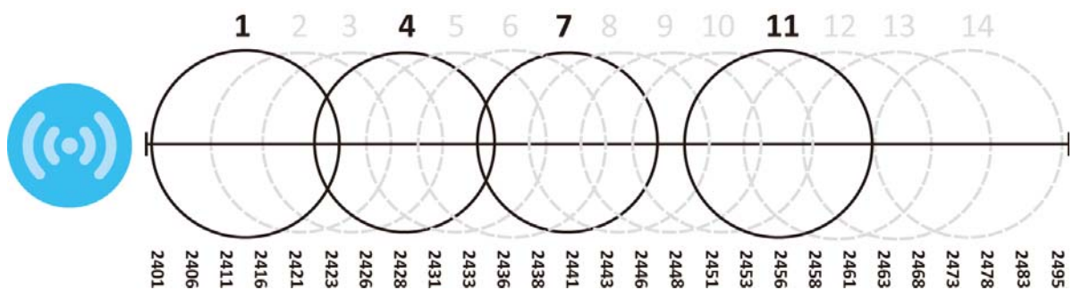
Figure 161 An Example Four-Channel Deployment
