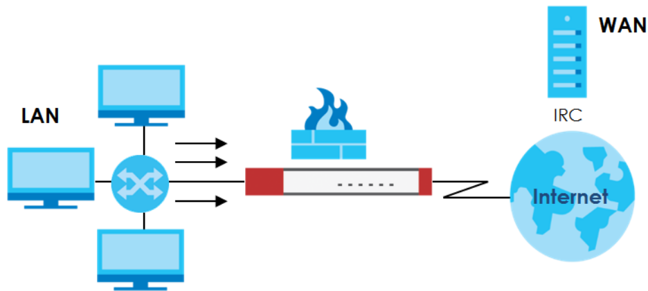
Figure 334 Blocking All LAN to WAN IRC Traffic Example
