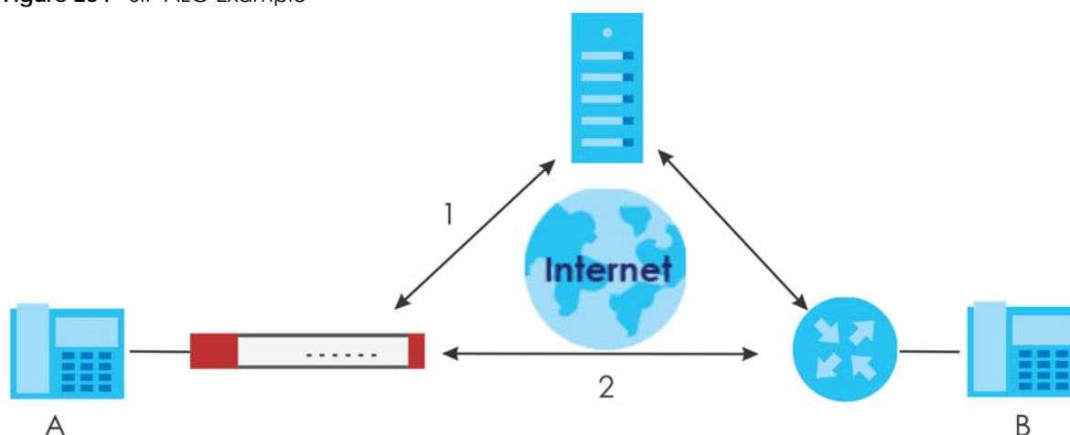
Figure 234 SIP ALG Example
