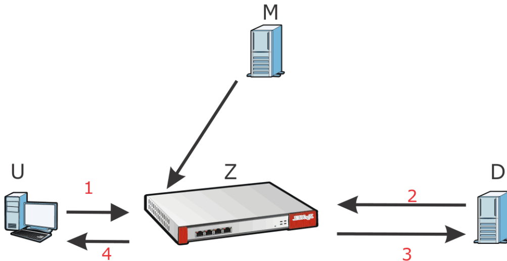
Figure 371 SSL Inspection Certificate Update Overview
