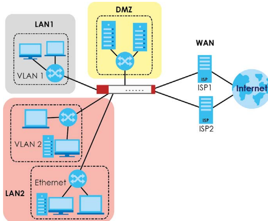
Figure 373 Example: Zones
