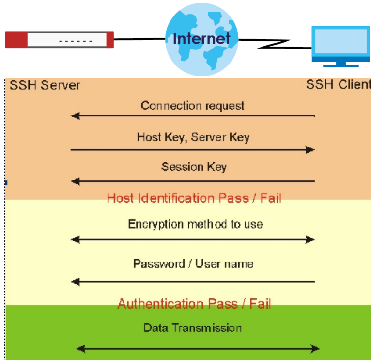
Figure 488 How SSH v1 Works Example
