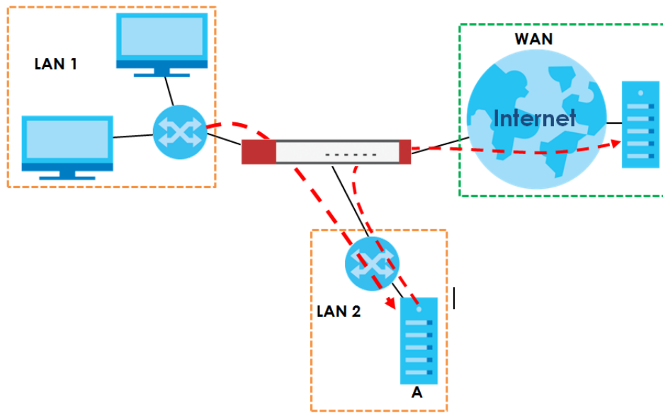
Figure 231 SMTP Redirect Example
