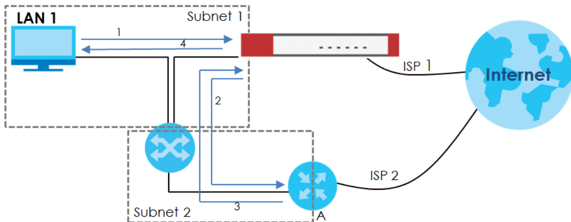
Figure 325 Using Virtual Interfaces to Avoid Asymmetrical Routes
