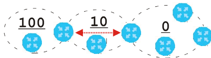
Figure 212 OSPF: Virtual Link
