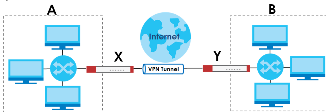
Figure 264 IPSec VPN Example
