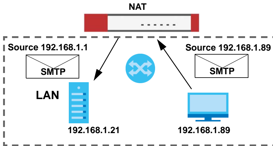
Figure 228 LAN to LAN Traffic
