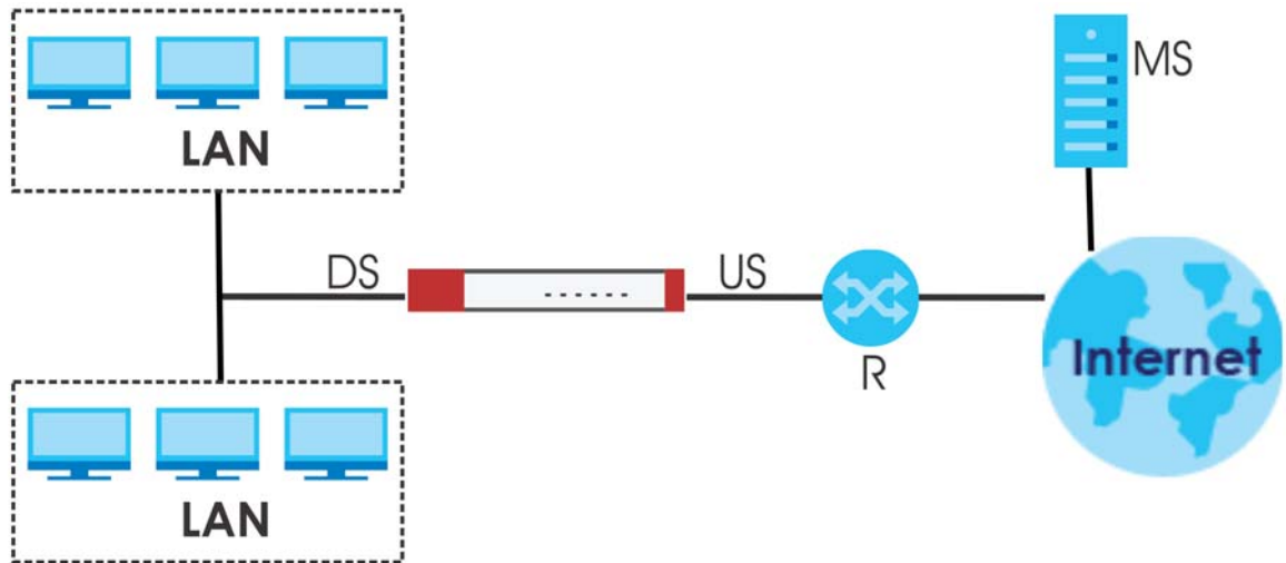
Figure 165 IGMP Proxy
