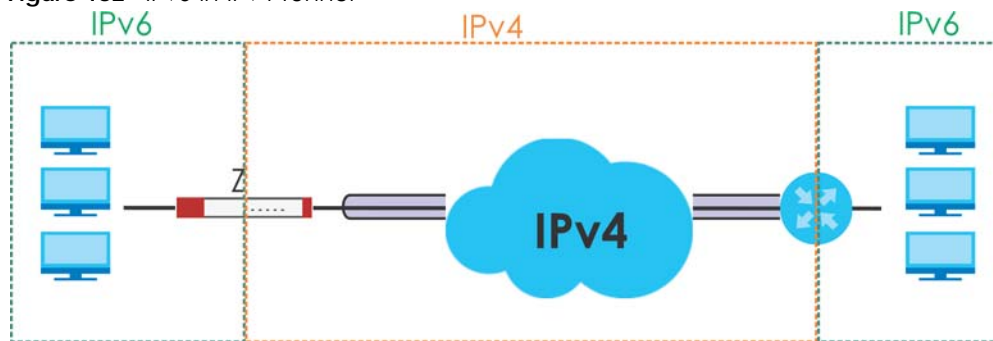
Figure 182 IPv6-in-IPv4 Tunnel
