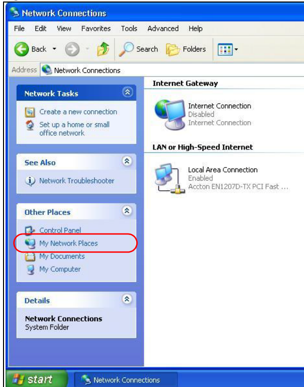
Figure 246 Network Connections
