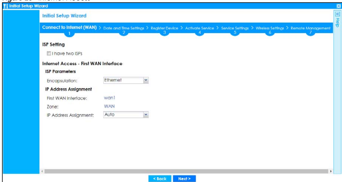
Figure 23 Internet Access
