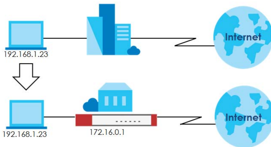
Figure 262 IPnP Application
