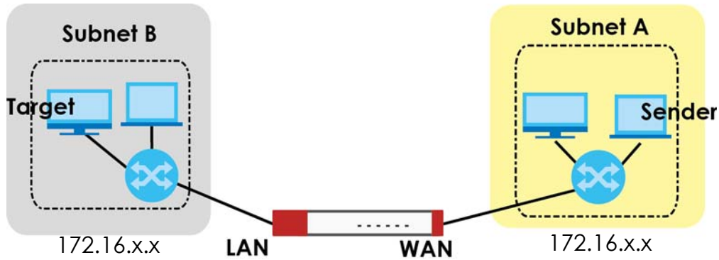
Figure 169 Proxy ARP
