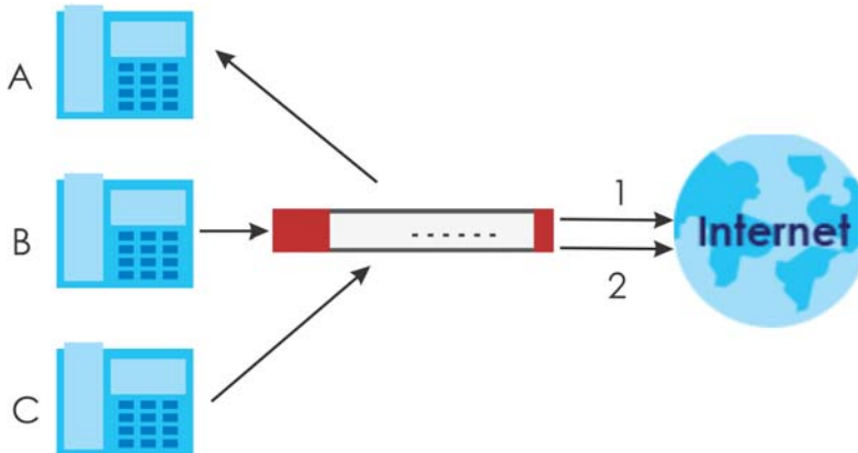
Figure 236 VoIP Calls from the WAN with Multiple Outgoing Calls
