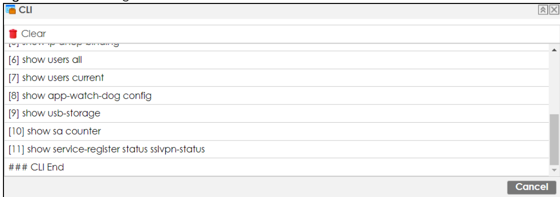
Figure 13 CLI Messages
