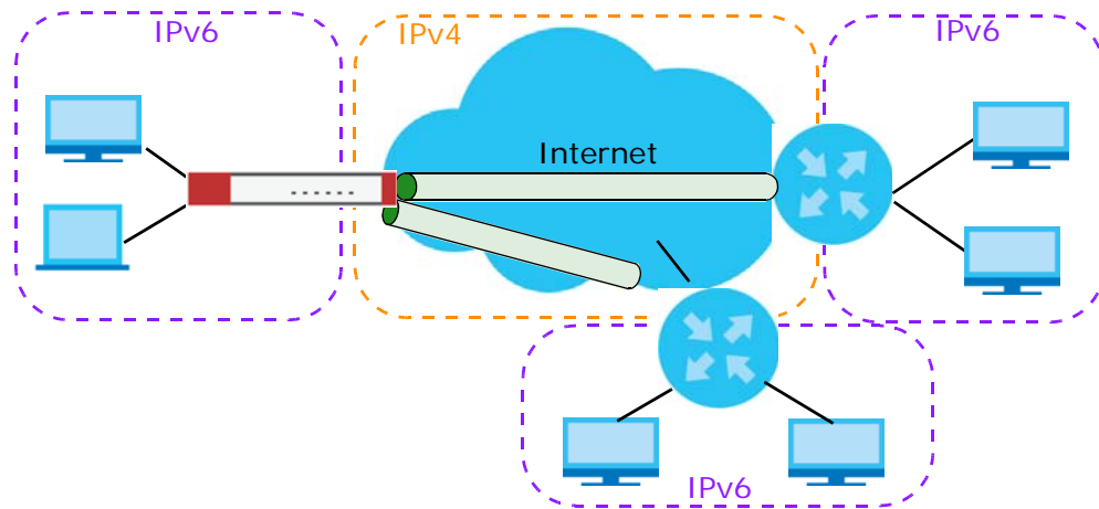
Figure 183 6to4 Tunnel
