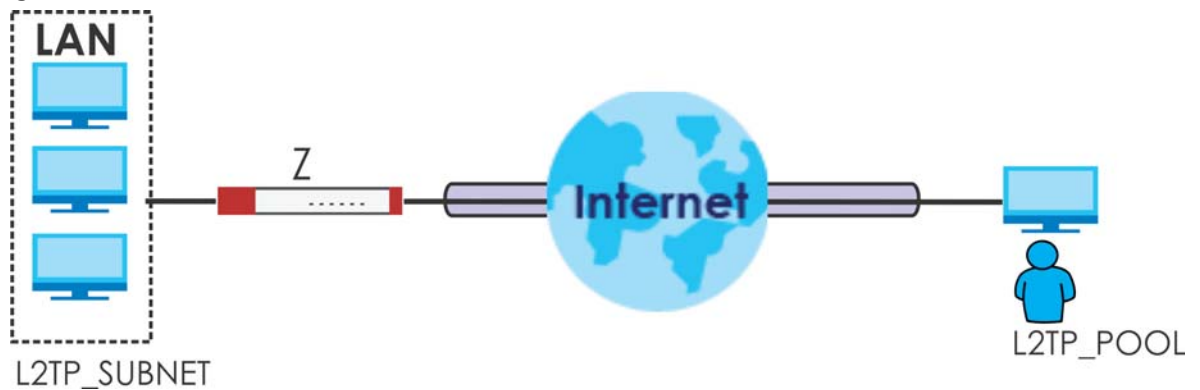
Figure 288 Policy Route for L2TP VPN
