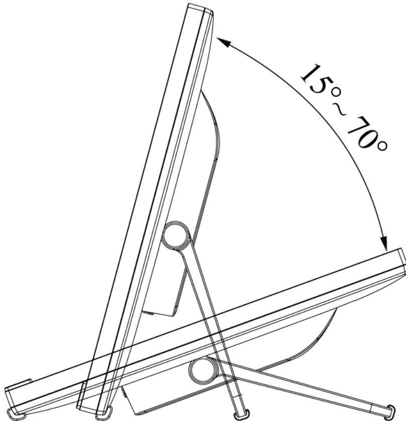
Figure.3. Monitor Angle
