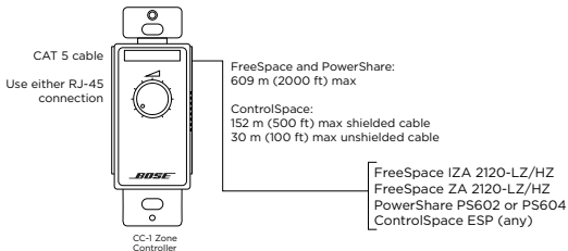
Either RJ-45 on CC-1 Zone Controller
