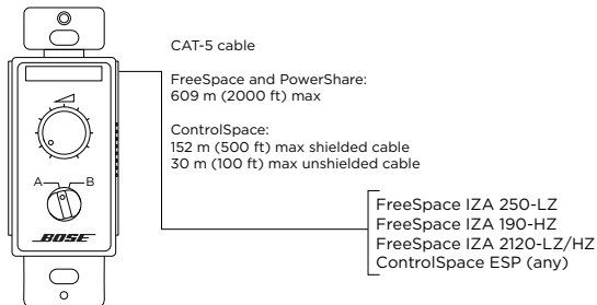
Either RJ-45 on CC-2 Zone Controller
