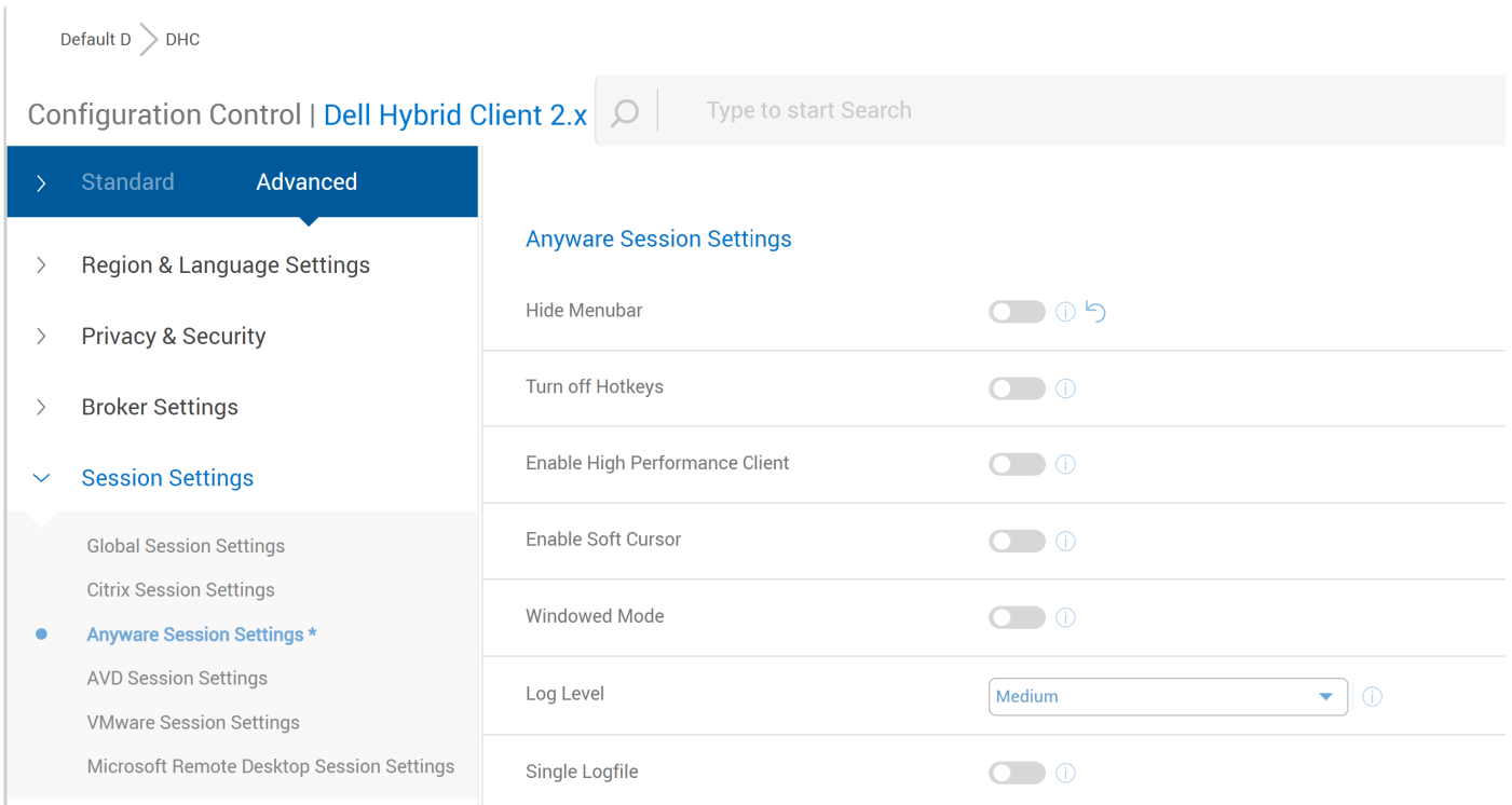
Figure 87. Single Logfile
