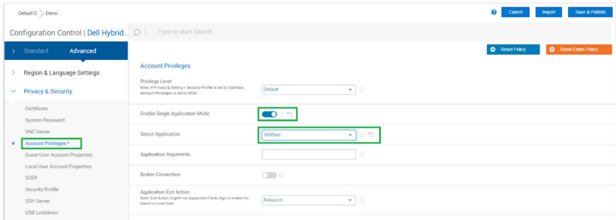
Figure 126. Account Privileges
