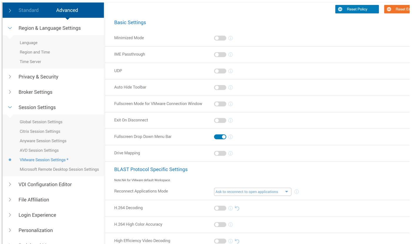
Figure 92. Basic and BLAST Protocol Specific Settings
