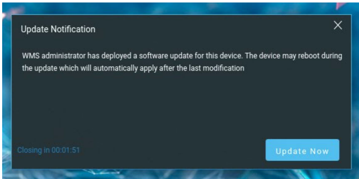
Figure 18. Update Notification
