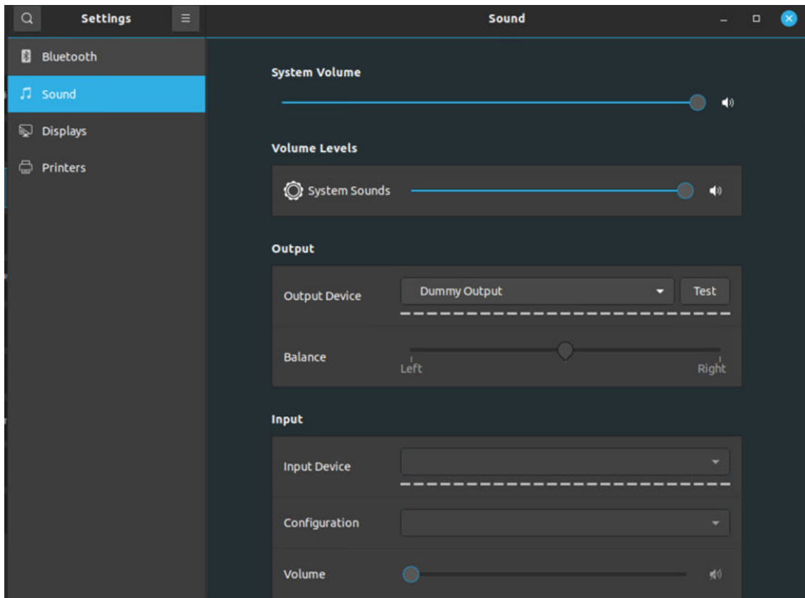
Figure 210. Sound
