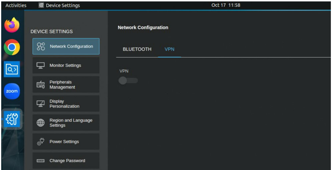
Figure 111. Network Configuration
