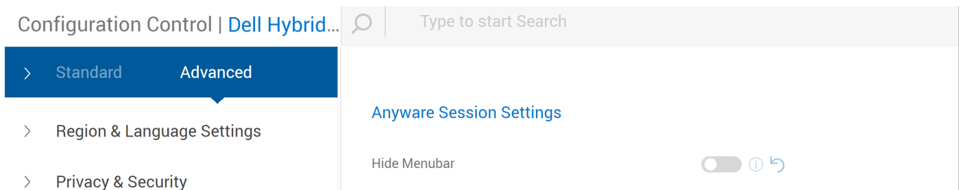
Figure 81. Hide Menubar
