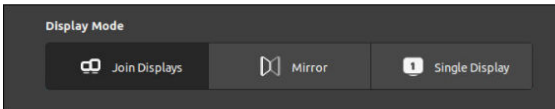
Figure 139. Display Mode
