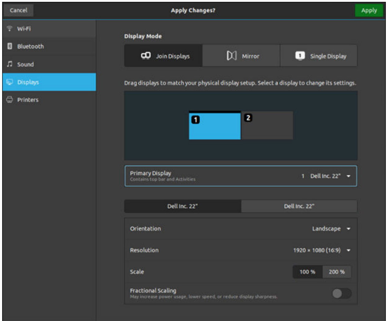
Figure 140. Join Display
