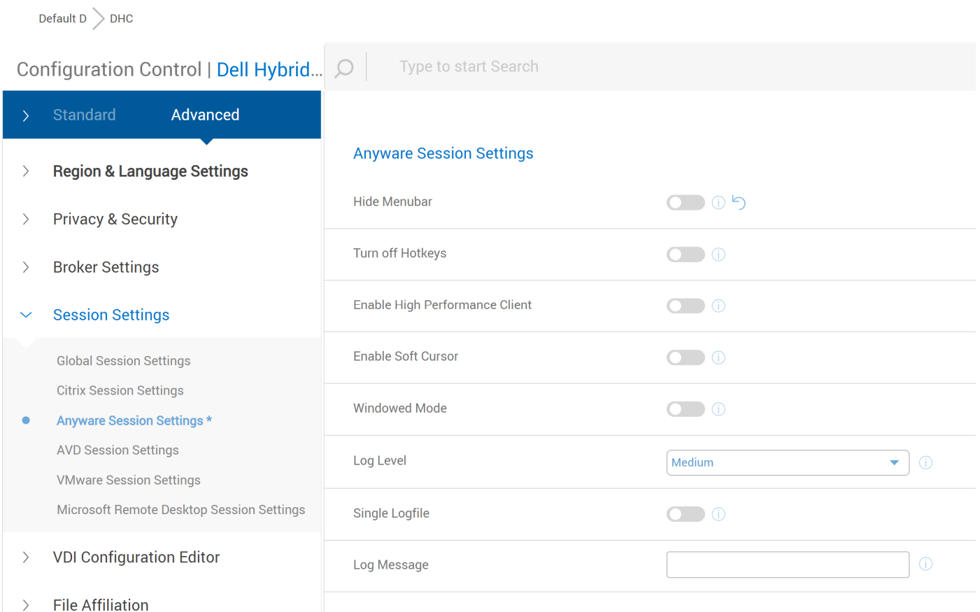
Figure 88. Log Message
