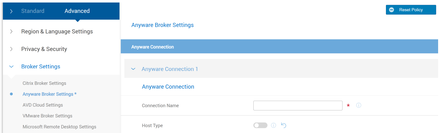
Figure 71. Host Type
