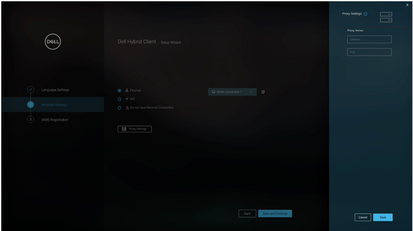
Figure 51. Proxy Settings
