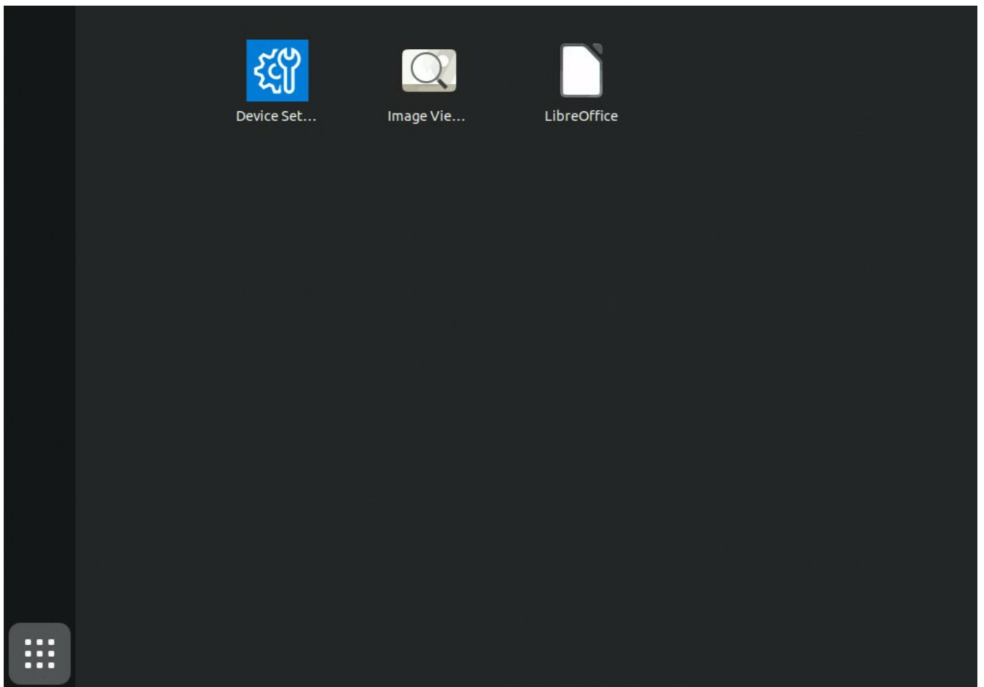
Figure 26. Show Application
