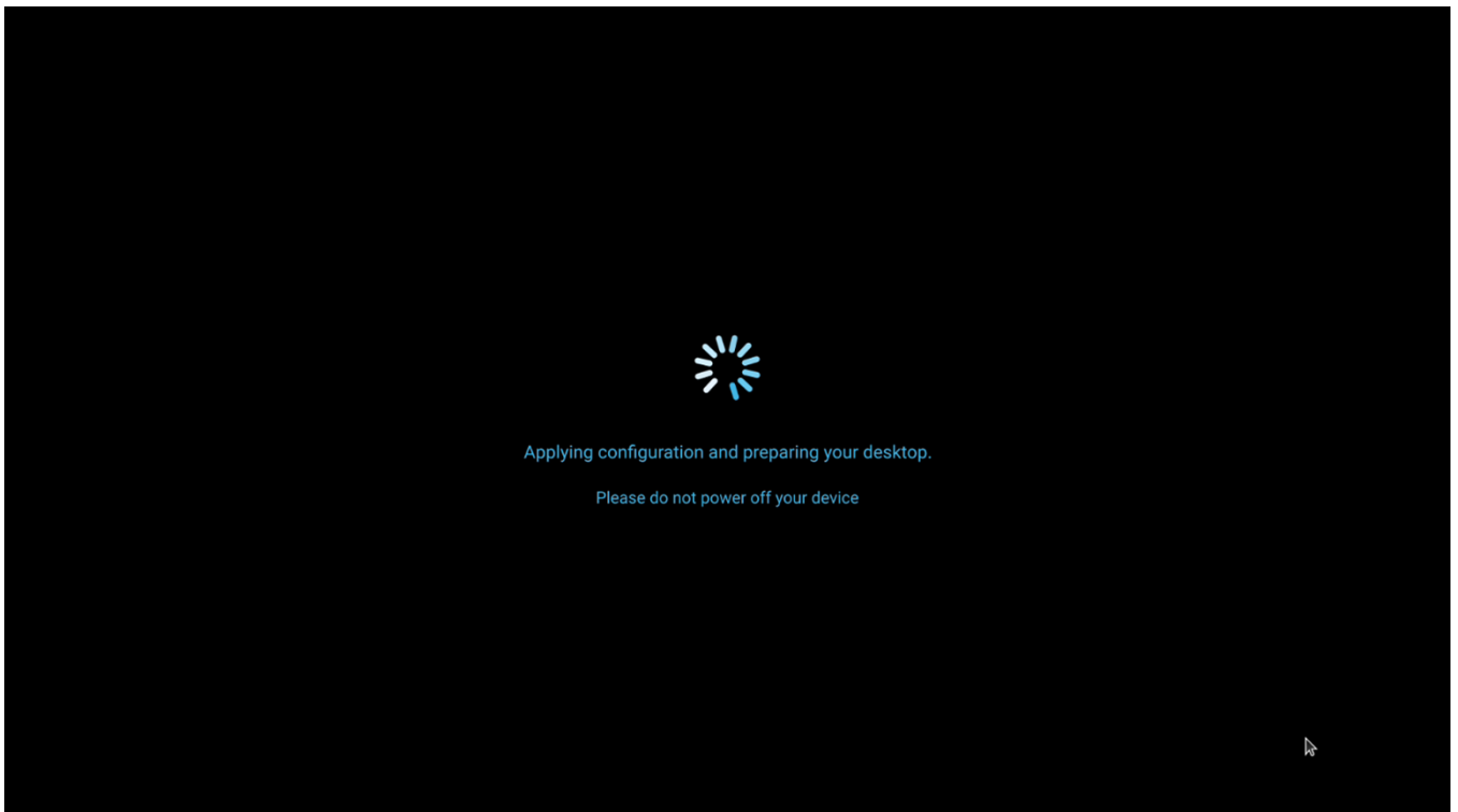
Figure 60. Apply Configuration
