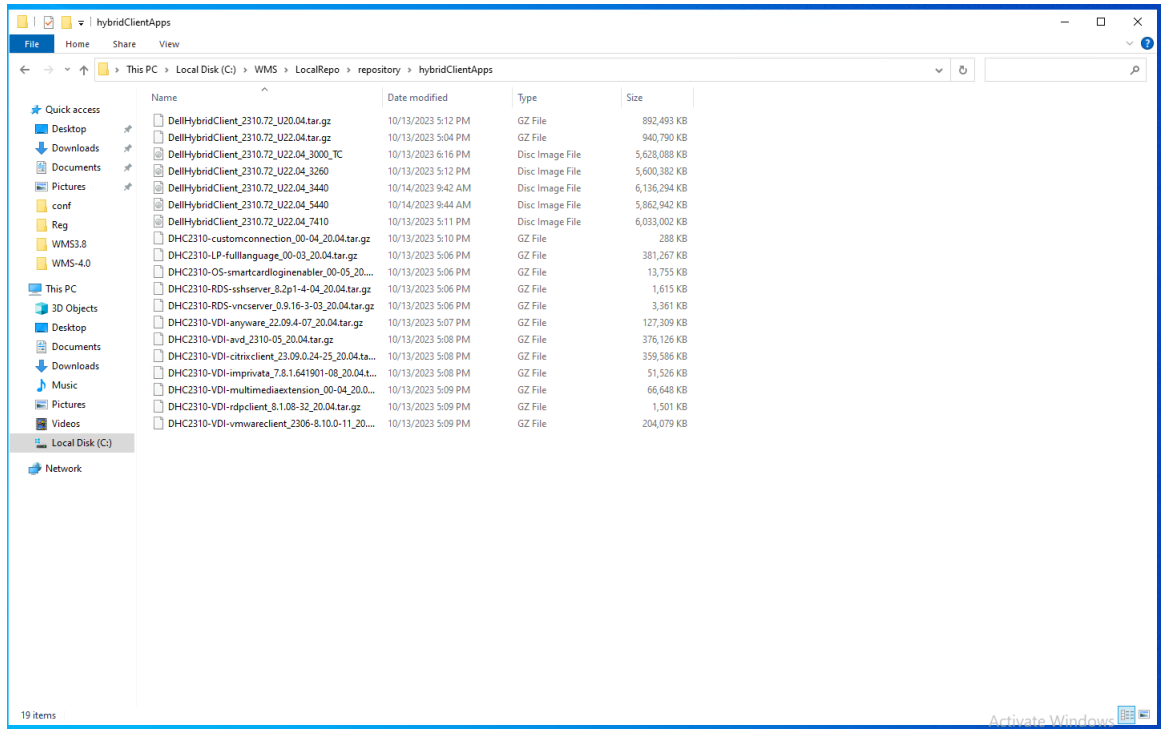
Figure 2. Local Repository
