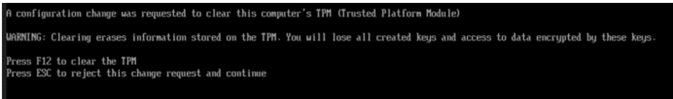
Figure 130. TPM Clear
