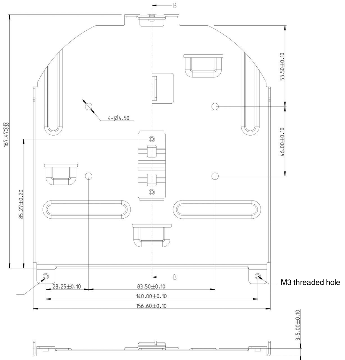
Metal plate B - ceiling side
