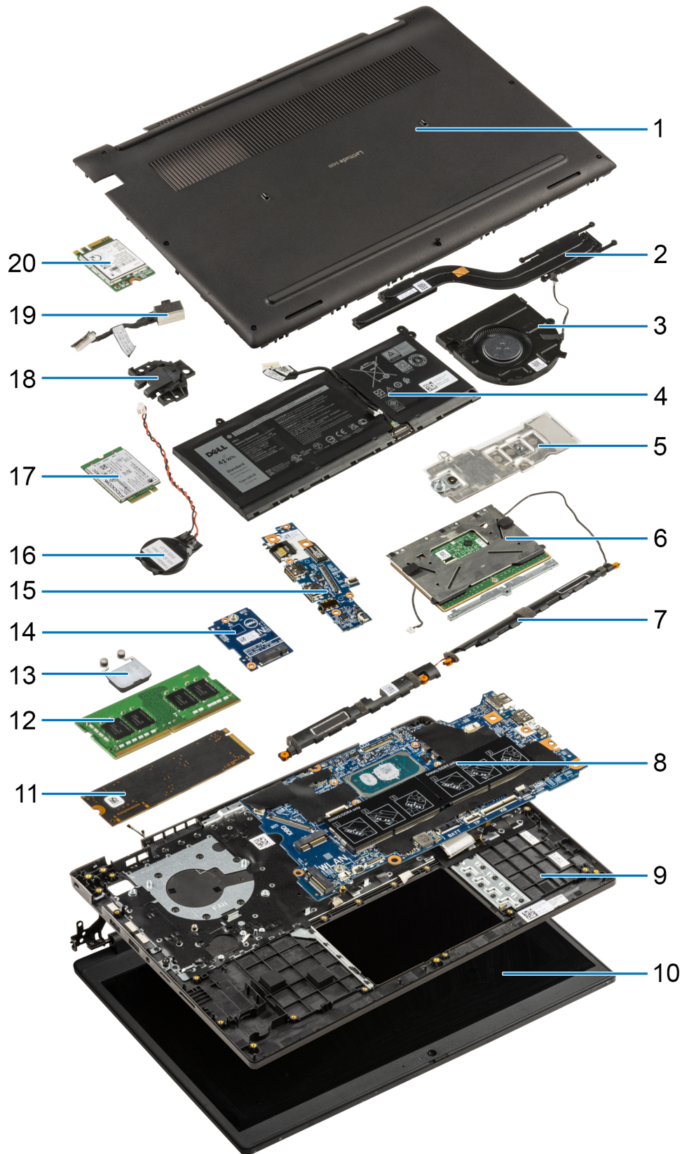
1. Base cover
