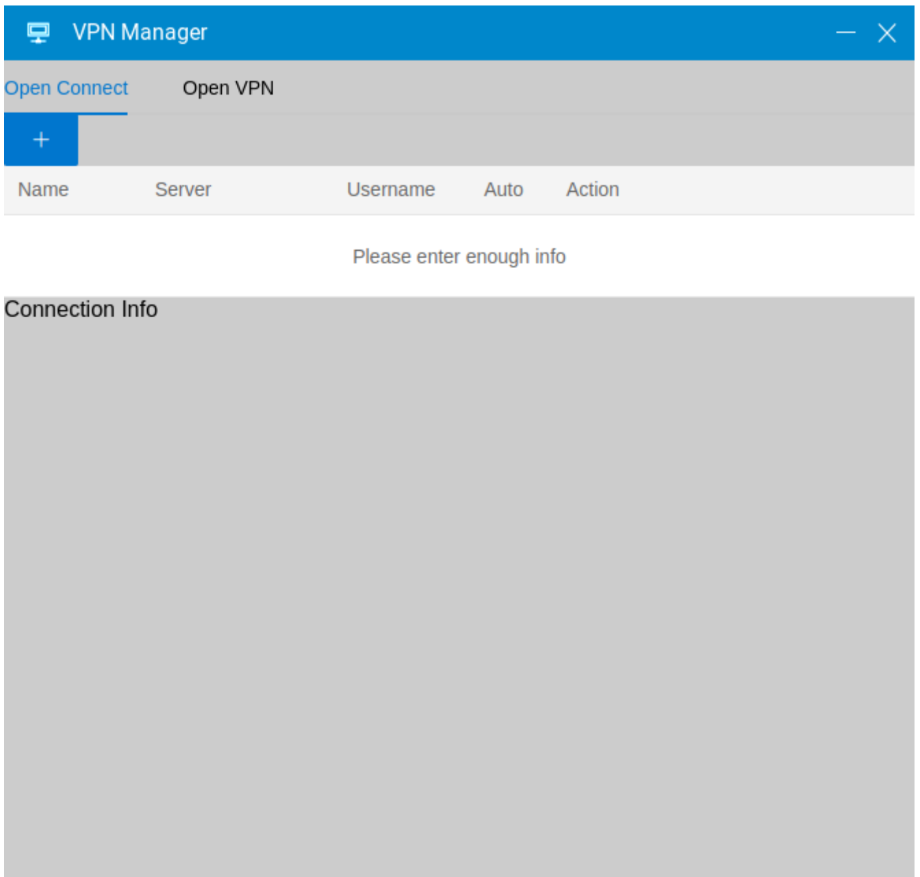
Figure 20. VPN Manager
