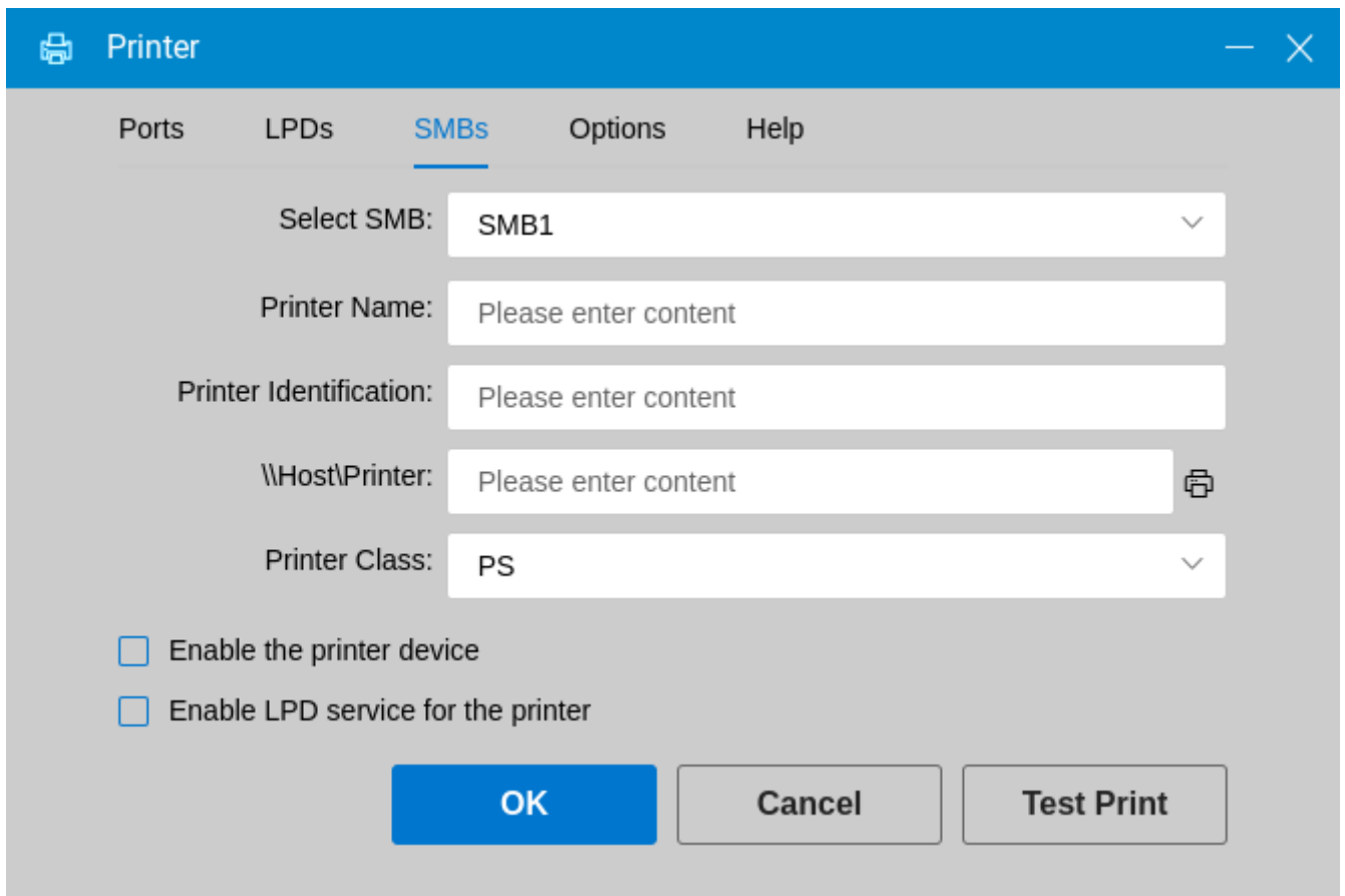
Figure 53. SMB
