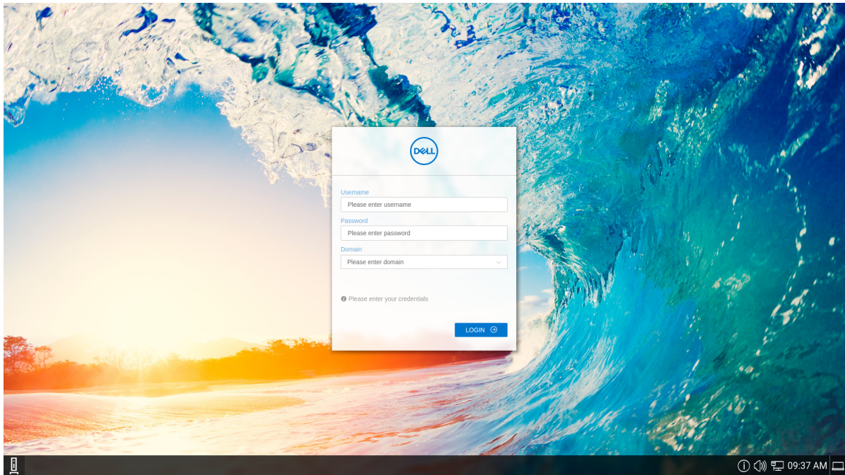
Figure 11. Classic Desktop
