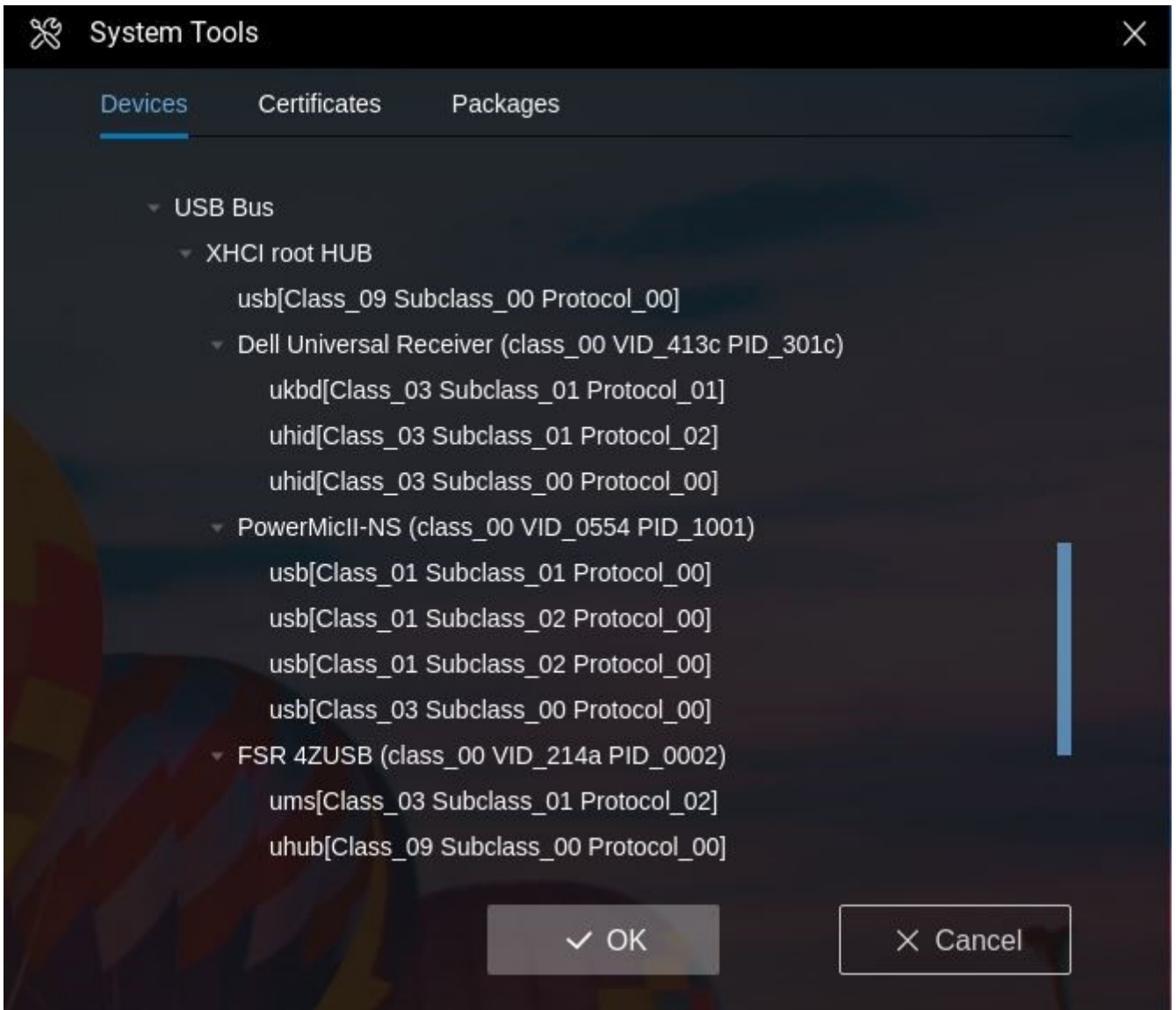
Figure 30. USB redirection
