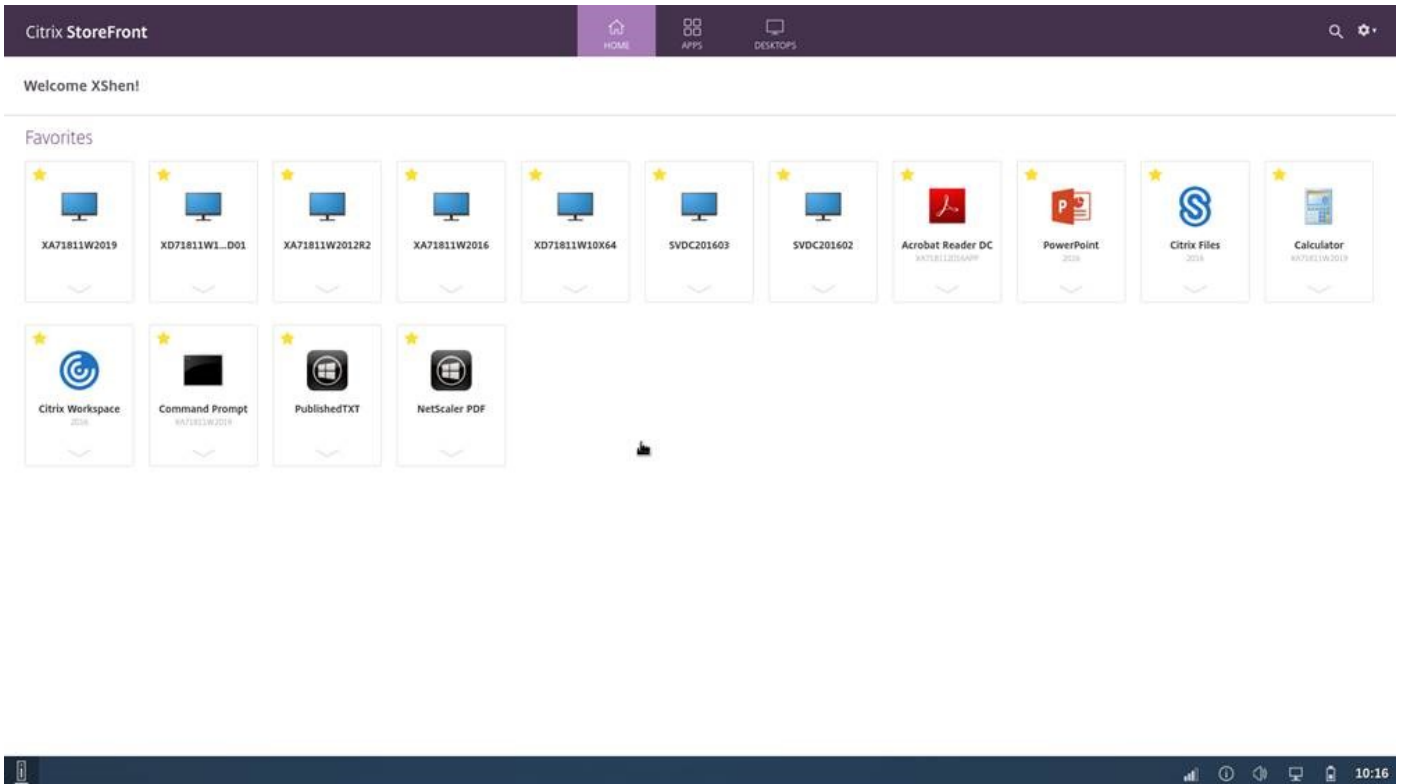
Figure 23. Workspace mode
