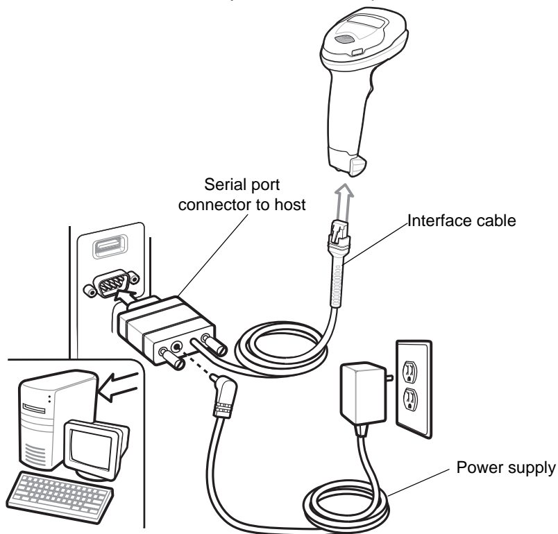
Figure 8-1 RS-232 Connection
