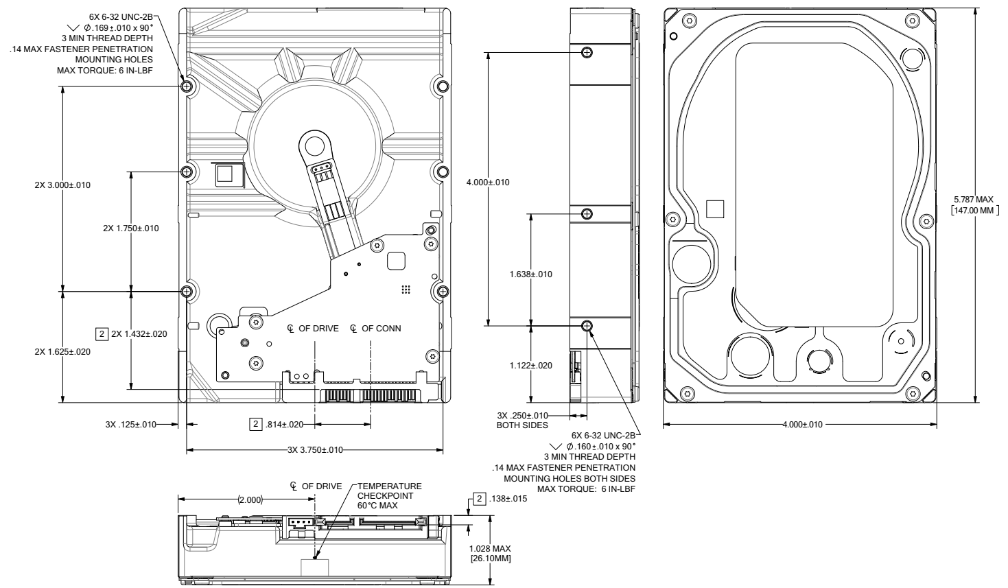
Figure 4. Mounting configuration dimensions 5-disk models
